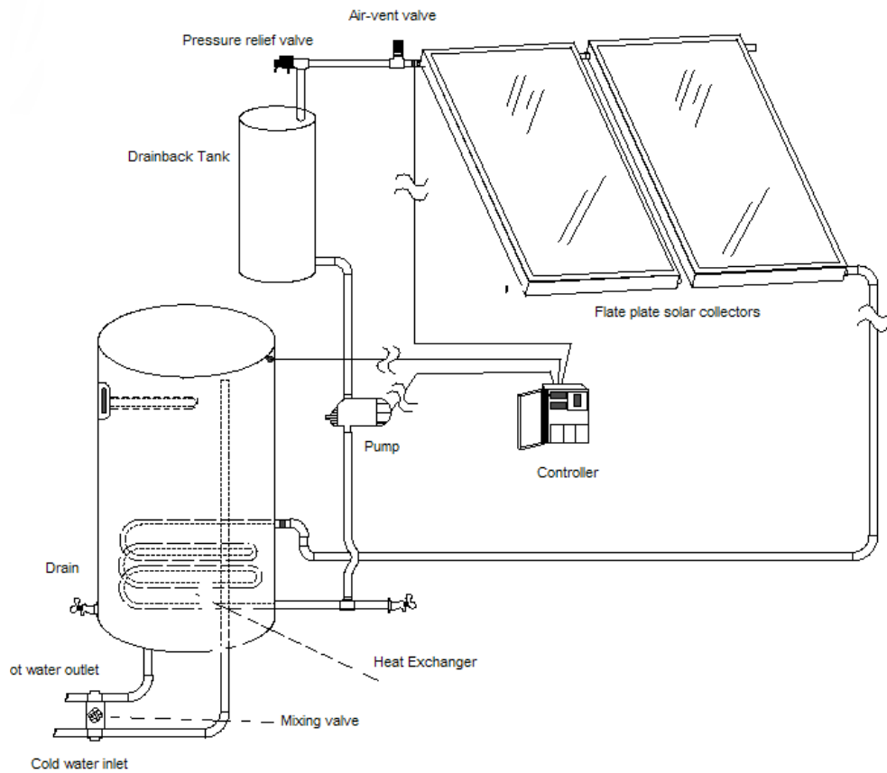
Figure (5). Drain-back solar water heating system
