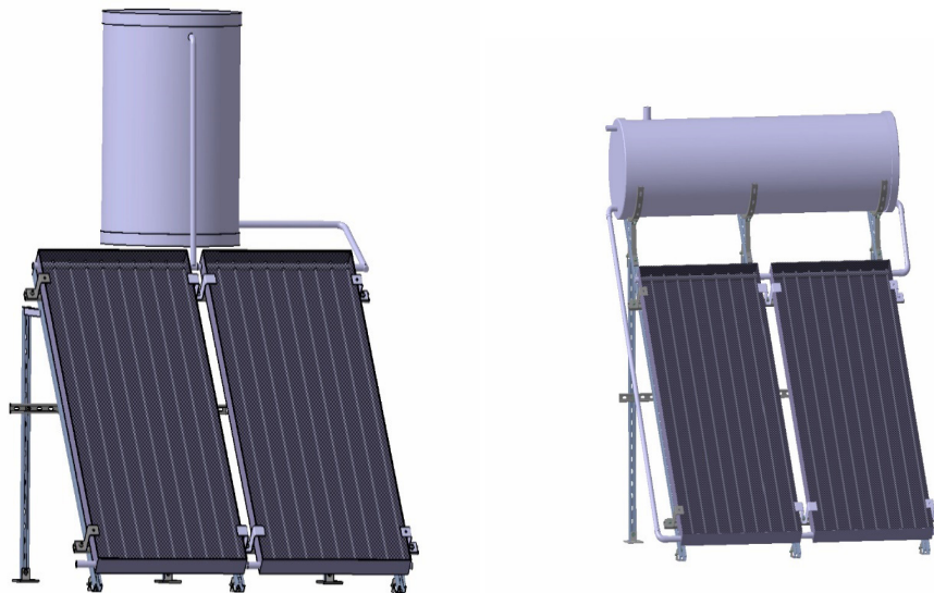
Figure (3). General view of the common thermosyphon solar water heating systems
